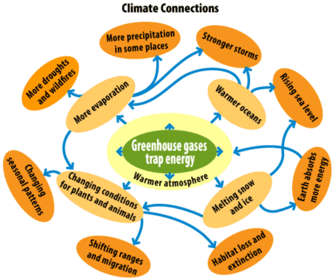
Figure 19: The complex connections contributing to Climate
